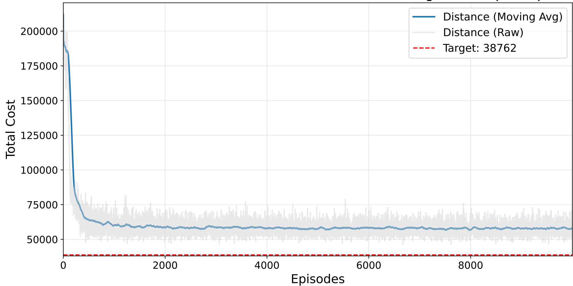
Final HYPERBAND GP Masked AutoRL-SOP Training - kro124p.1.sop
